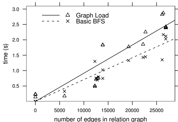
Figure 11. For queries issued during a 6-month trace of the author’s system: the time spent loading the relation graph and the execution time of the basic BFS algorithm against the number of edges in the relation graph. (5 trials per query; standard deviations were within 2% of the mean for each data point.)
