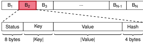
Figure 7: Hash-Table Data Structure – An overview of the DBMS’s open-addressing hash-table used for joins (with B_N buckets).
