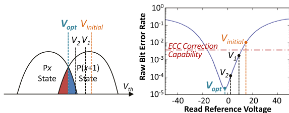
Fig. 23. Finding the optimal read reference voltage after the threshold voltage distributions overlap (left), and raw bit error rate as a function of the selected read reference voltage (right).
