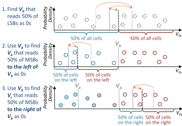
Fig. 24. Disparity-based read reference voltage approximation to find V_{initial} for MLC NAND flash memory. Each circle represents a cell, where a dashed border indicates that the LSB is undetermined, a solid border indicates that the LSB is known, a hollow circle indicates that the MSB is unknown, and a filled circle indicates that the MSB is known.
