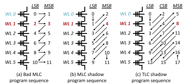
Fig. 20. Order in which the pages of each wordline (WL) are programmed using (a) a bad programming sequence, and using shadow sequencing for (b) MLC and (c) TLC NAND flash. The bold page programming operations for WL1 induce cell-to-cell program interference when WL0 is fully programmed.
