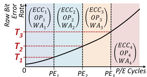
Fig. 27. Illustration of how multi-rate ECC switches to different ECC codewords (i.e., ECC_i ) as the RBER grows. OP_i is the overprovisioning factor used for engine ECC_i , and WA_i is the resulting write amplification value.
