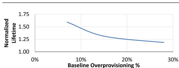
Fig. 28. Lifetime improvements of using multi-rate ECC over using a fixed ECC coding rate.
