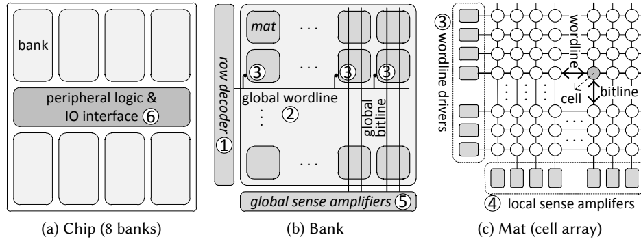
Fig. 2. Hierarchical Organization of a DRAM System
