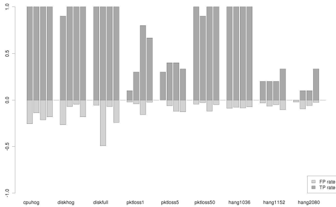
Fig. 6. Results for all problems on RandWriter for all cluster sizes.
