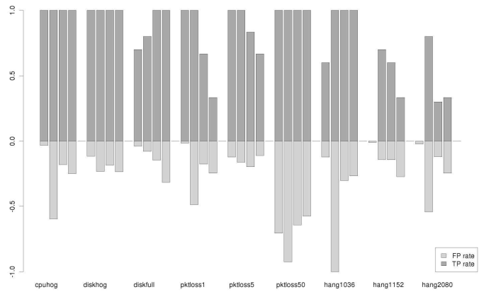
Fig. 4. Results for all problems on Nutch for all cluster sizes.
