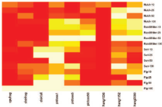
Fig. 9. False-negative rates for all problem-workload pairs (Maps).
