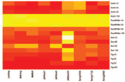
Fig. 10. False-positive rates for all problem-workload pairs (all other states).
