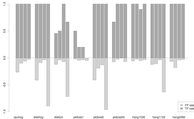
Fig. 7. Results for all problems on Sort for all cluster sizes.
