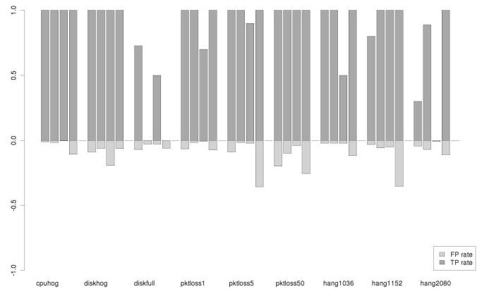
Fig. 5. Results for all problems on Pig for all cluster sizes.
