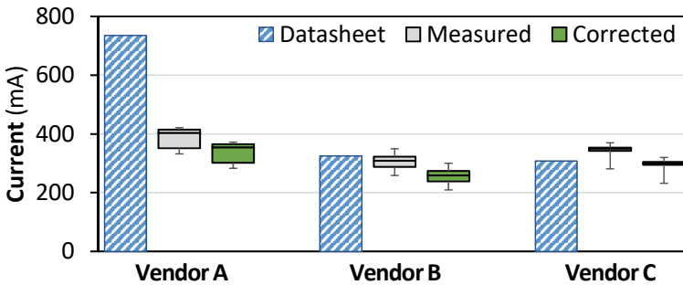
Fig. 10. IDD4R current measurements before and after correction for I/O driver current.
