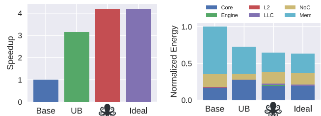
Figure 13: PHI results for PageRank on a 16M vertex, 160M edge synthetic graph. tākō improves performance by 4.2×.
