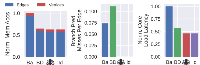
Figure 17: HATS performance breakdown. Left: DRAM accesses split by PageRank phase. Mid: core branch mispredictions per graph edge processed. Right: cumulative core load latency.
